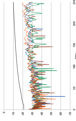
Return Loss Cassette to Outlet
